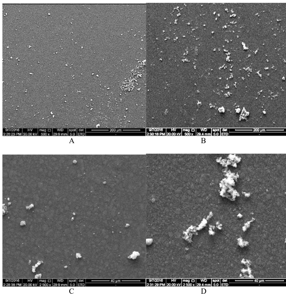
Figure 3. SEM results. Nanofilled composite resin with 500x (A) and 2500x (C) magnification. Nanohybrid composite resin with 500x (B) and 2500x (D) magnification
